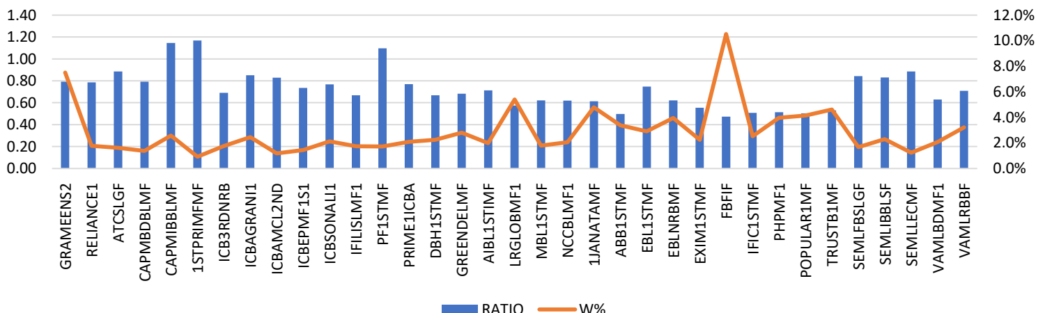
Price/N.A.V Ratio
